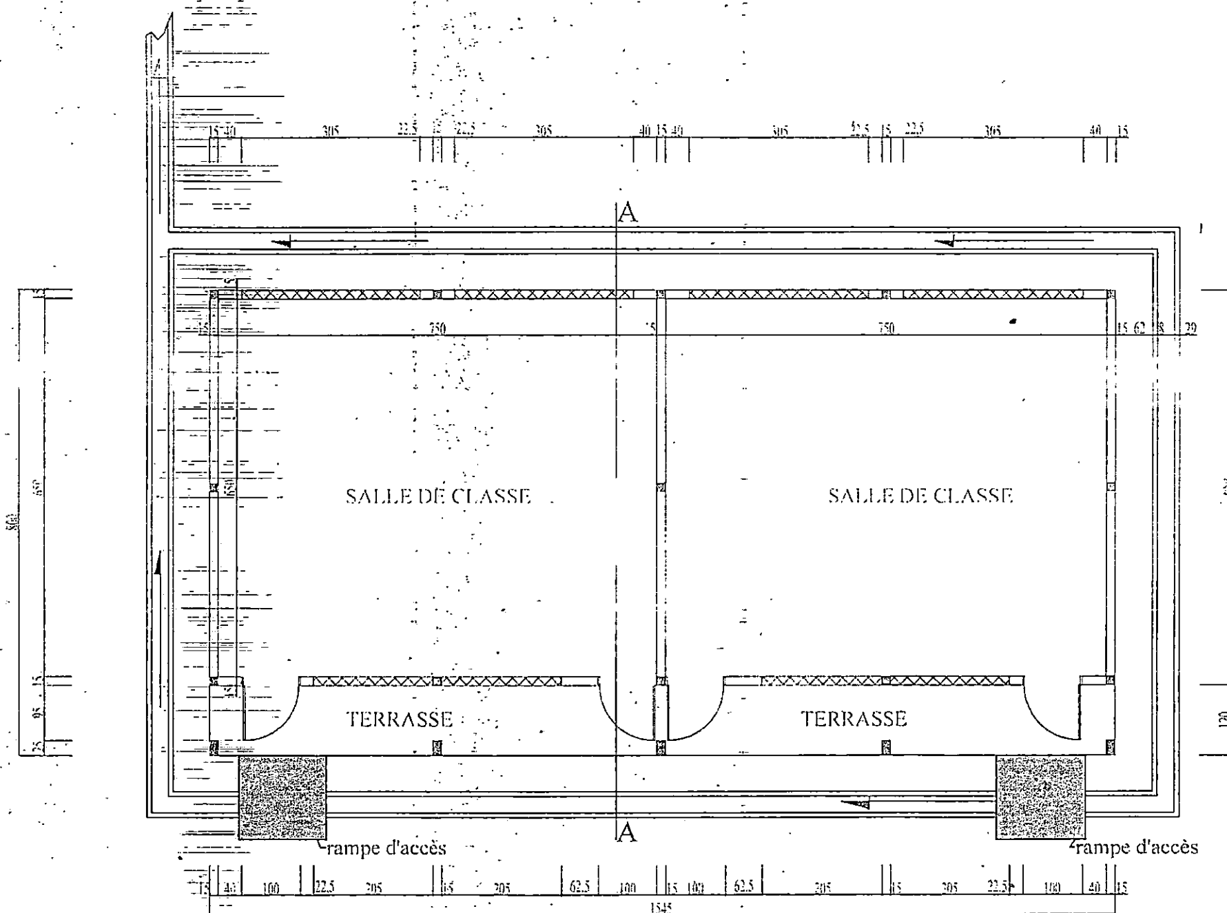
DISTRIBUTION PLAN
