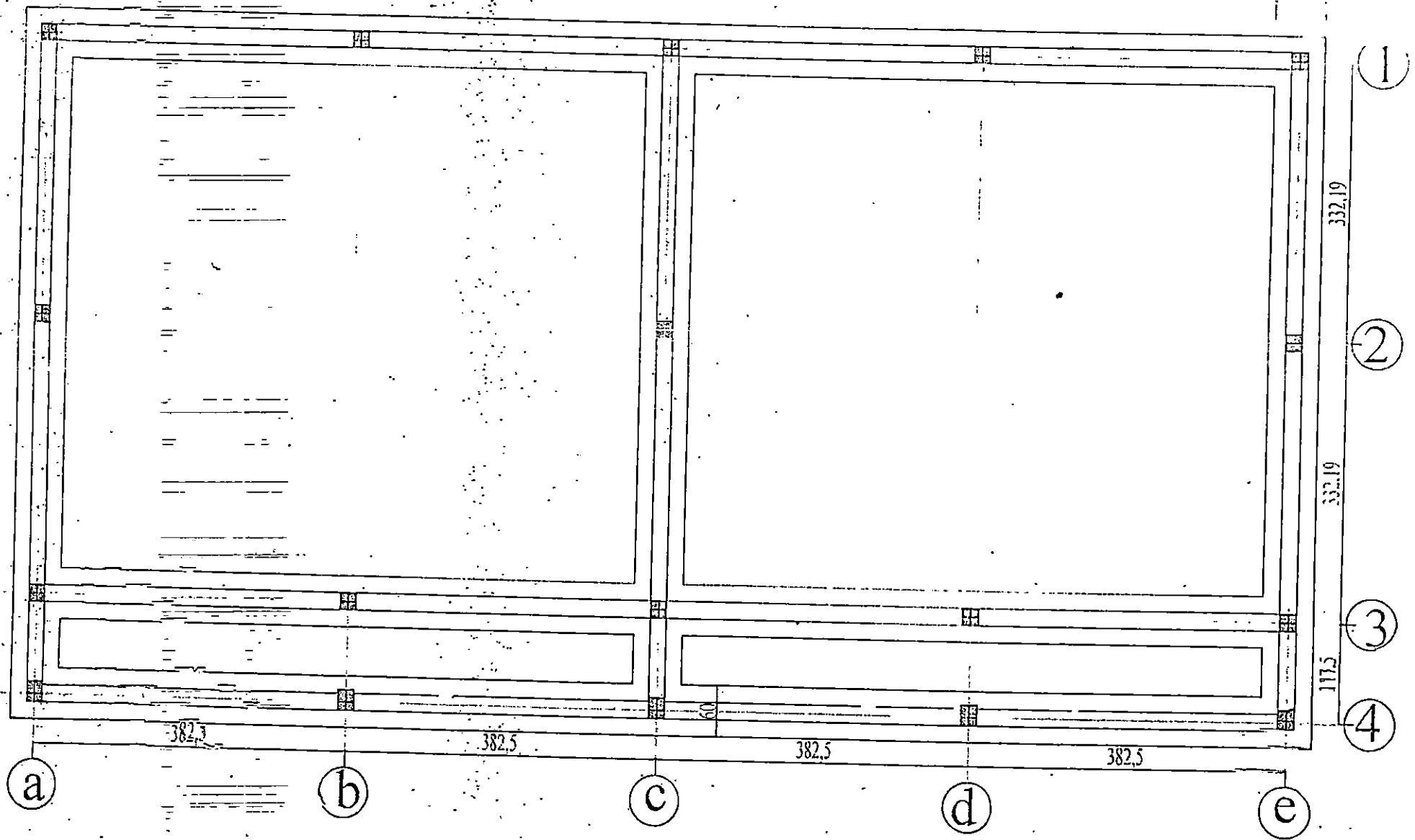
FOUNDATION PLAN
